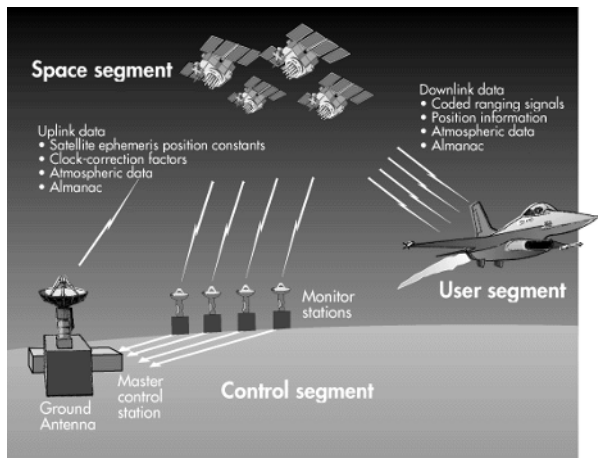
Figure 3-1: GPS is composed of satellites, ground stations, and receivers.
